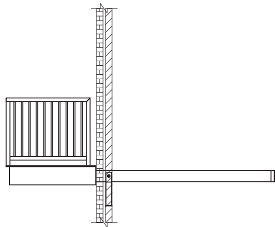
Face mounted, side view (above) Cantilevered mount, side view (below)
