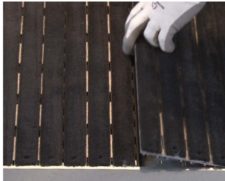
8 Join modules together by placing the aluminum foot into the black connector.
