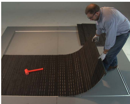
10 Continue to install the remaining modules.
