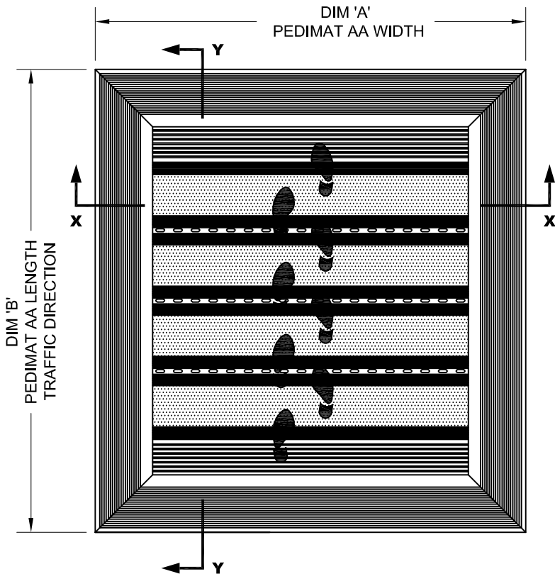
TYPICAL PLAN VIEW
