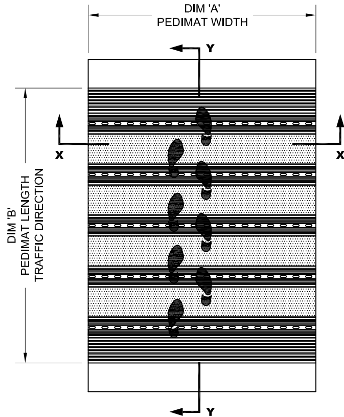
TYPICAL PLAN VIEW
