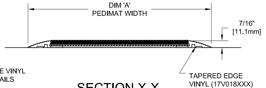
SECTION X-X
