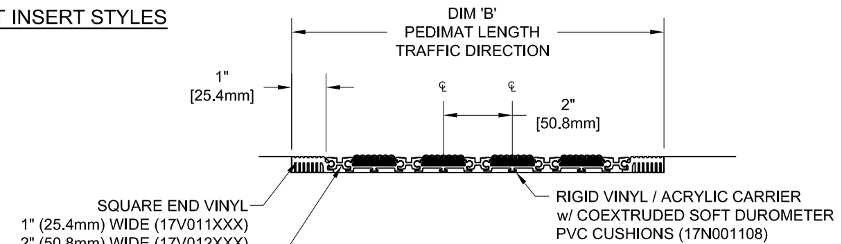
SECTION Y-Y
