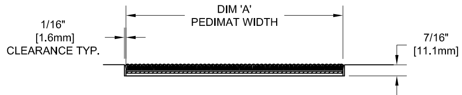
SECTION X-X
