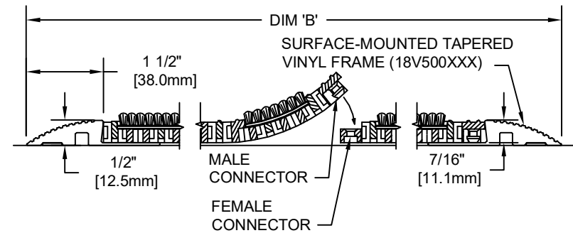
SECTION Y-Y
