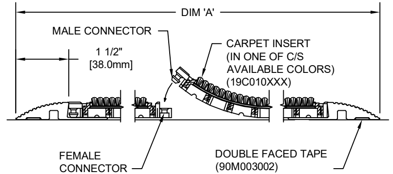
SECTION X-X
