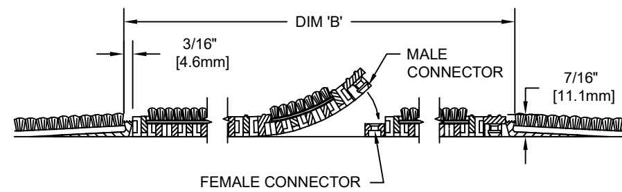
SECTION Y-Y
