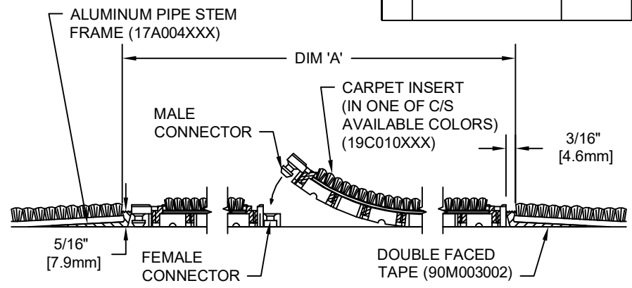
SECTION X-X
