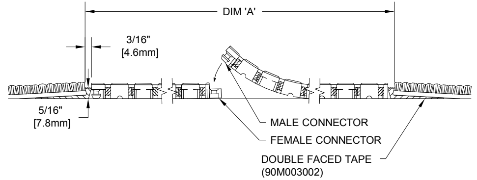
SECTION X-X
