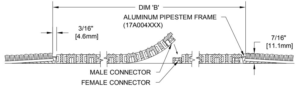
SECTION Y-Y
