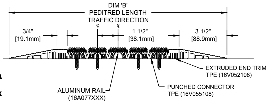
SECTION Y-Y
