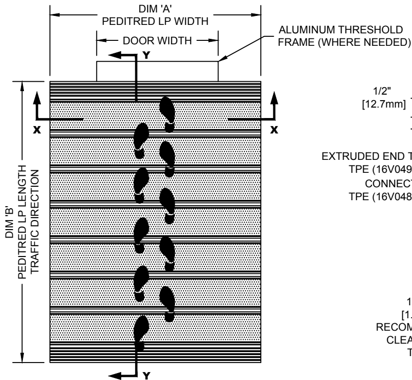
TYPICAL PLAN VIEW
