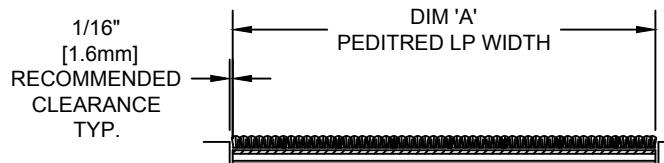
SECTION X-X
