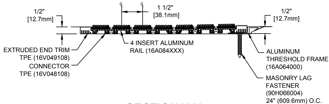
SECTION Y-Y
