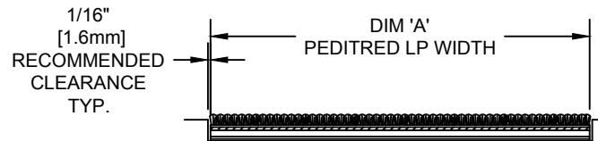
SECTION X-X
