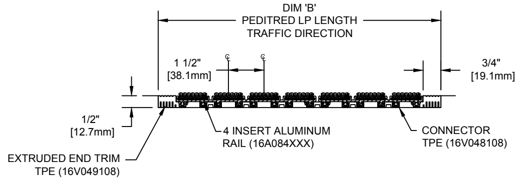
SECTION Y-Y
