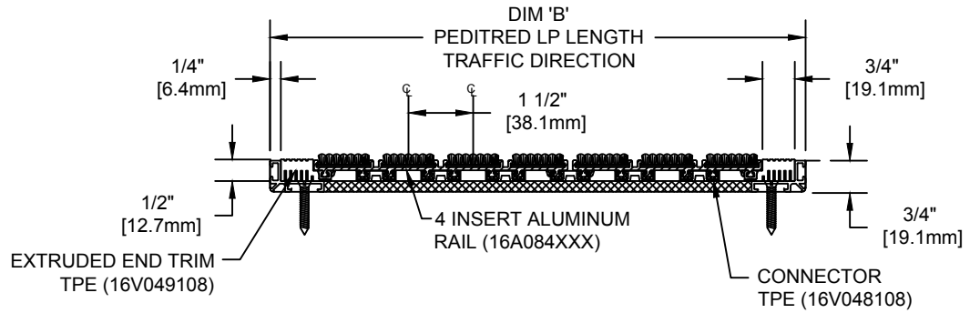
SECTION Y-Y
