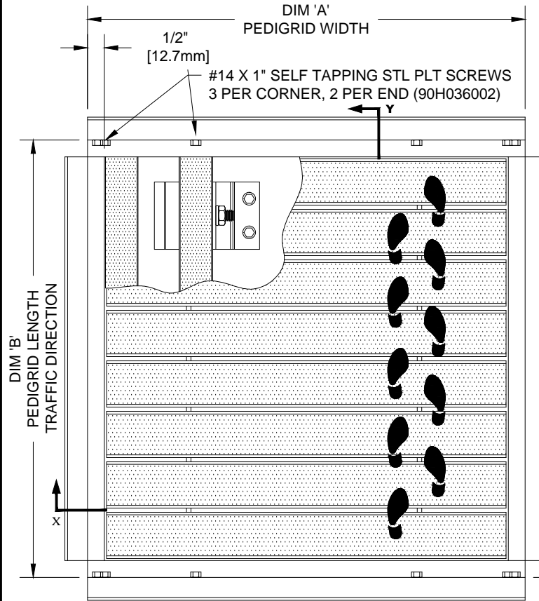
TYPICAL PLAN VIEW
