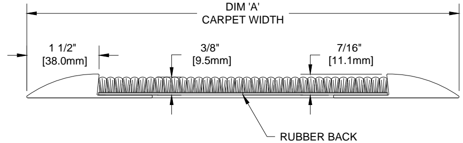
SECTION X-X
