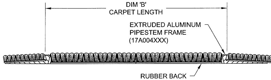
SECTION Y-Y
