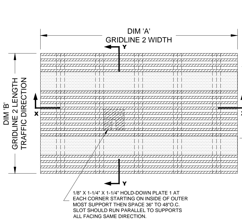
TYPICAL PLAN VIEW
