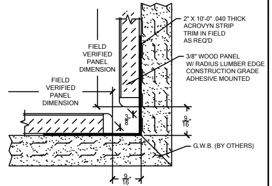
INSIDE CORNER CONDITION
