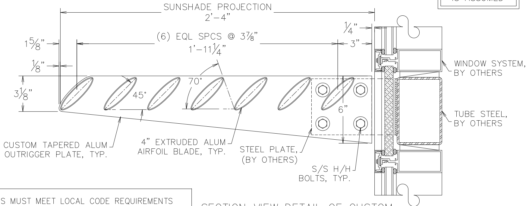
SECTION VIEW DETAIL OF CUSTOM CANTILEVER AIRFOIL SUNSHADE SYSTEM 100-3C-5
