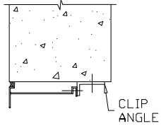
VERTICAL SECTION OF HEAD (for RS models)
