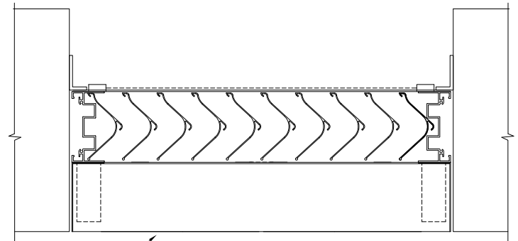
PLAN VIEW OF JAMBS WITH BLADE
