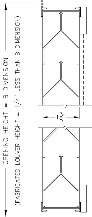
VERTICAL SECTION
