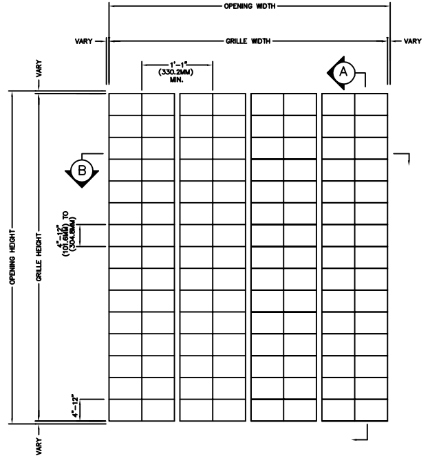
EXTERIOR ELEVATION
