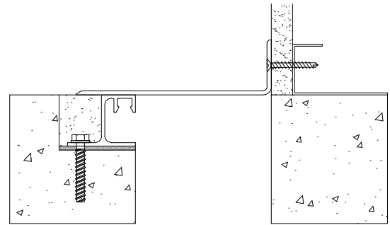
2" - 6" FINAL ASSEMBLY
