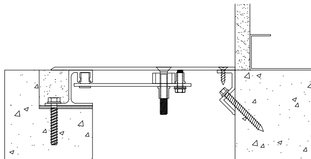
2" - 6" FINAL ASSEMBLY
