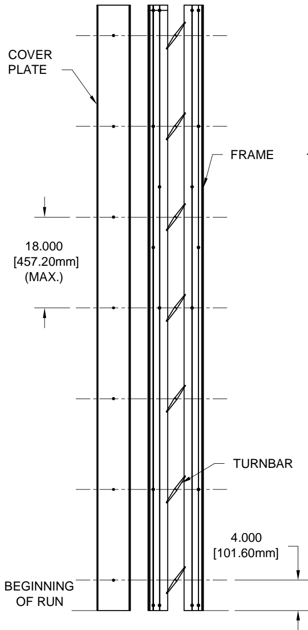
TURNBAR LOCATION
