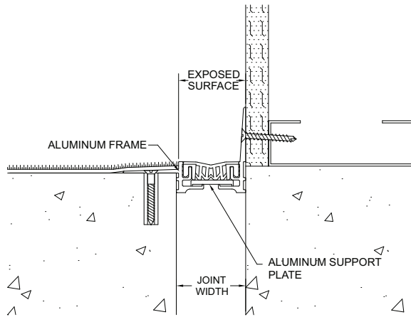
GFPSW-100
