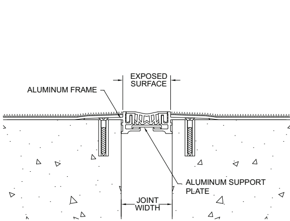
GFPS-100
