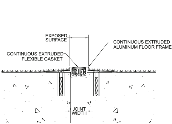
GFPS-100
