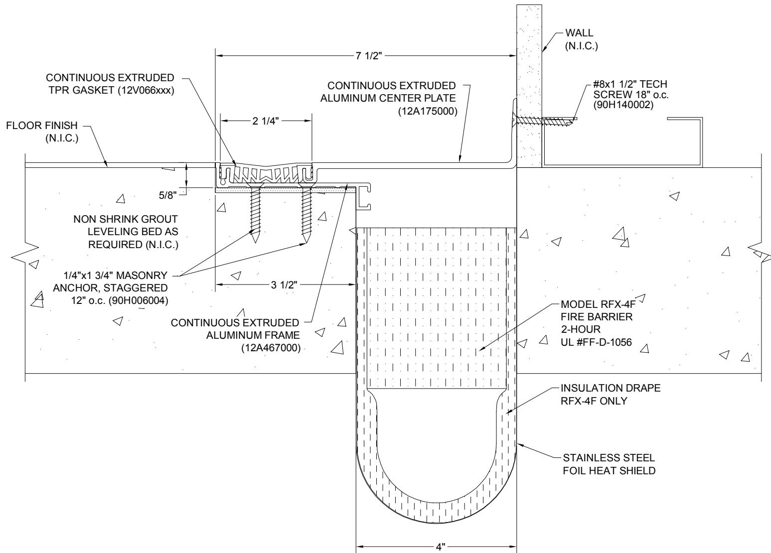
GTPW-400 w/ RFX4F
