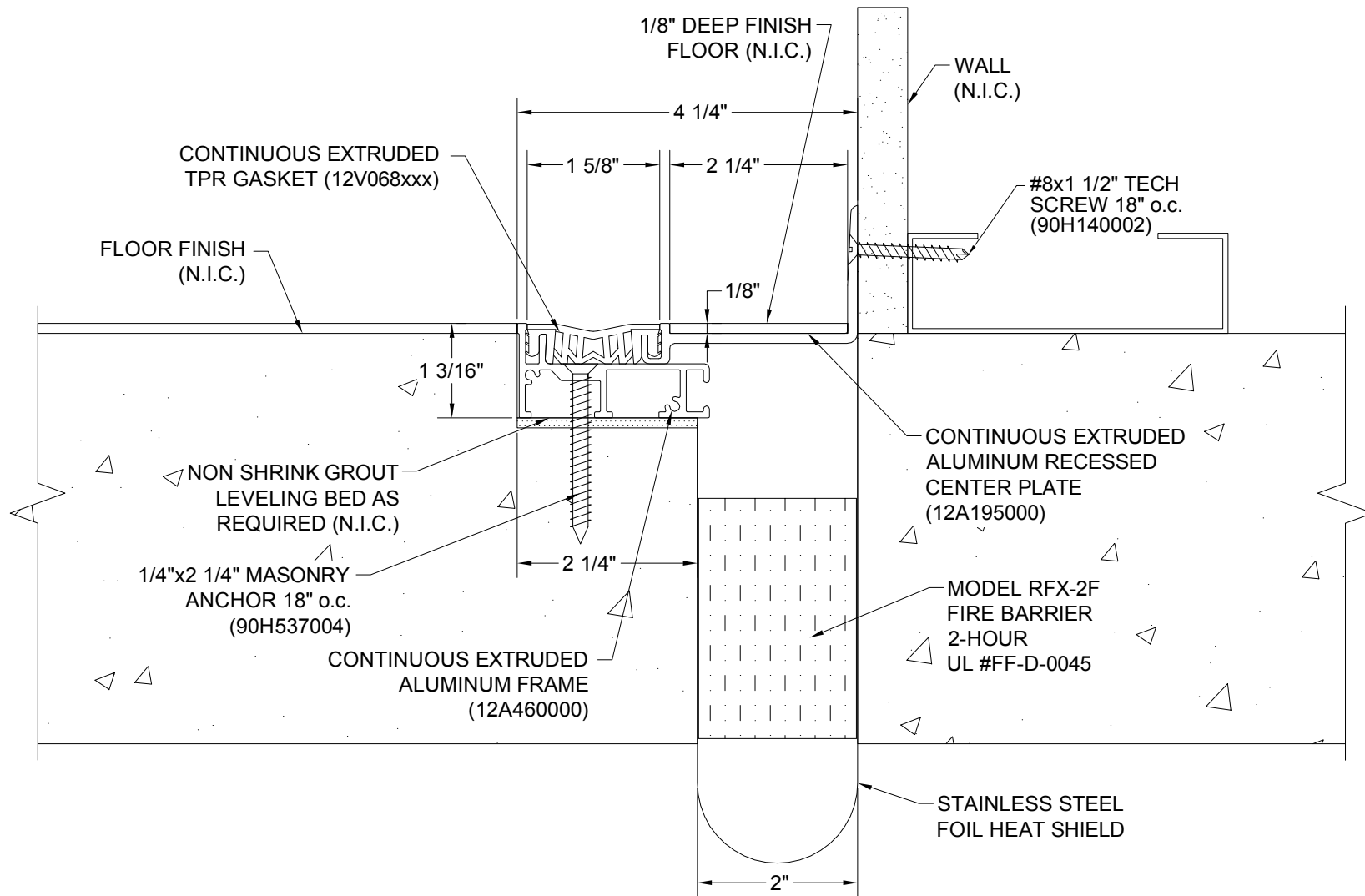
DGTRW-200 w/ RFX2F
