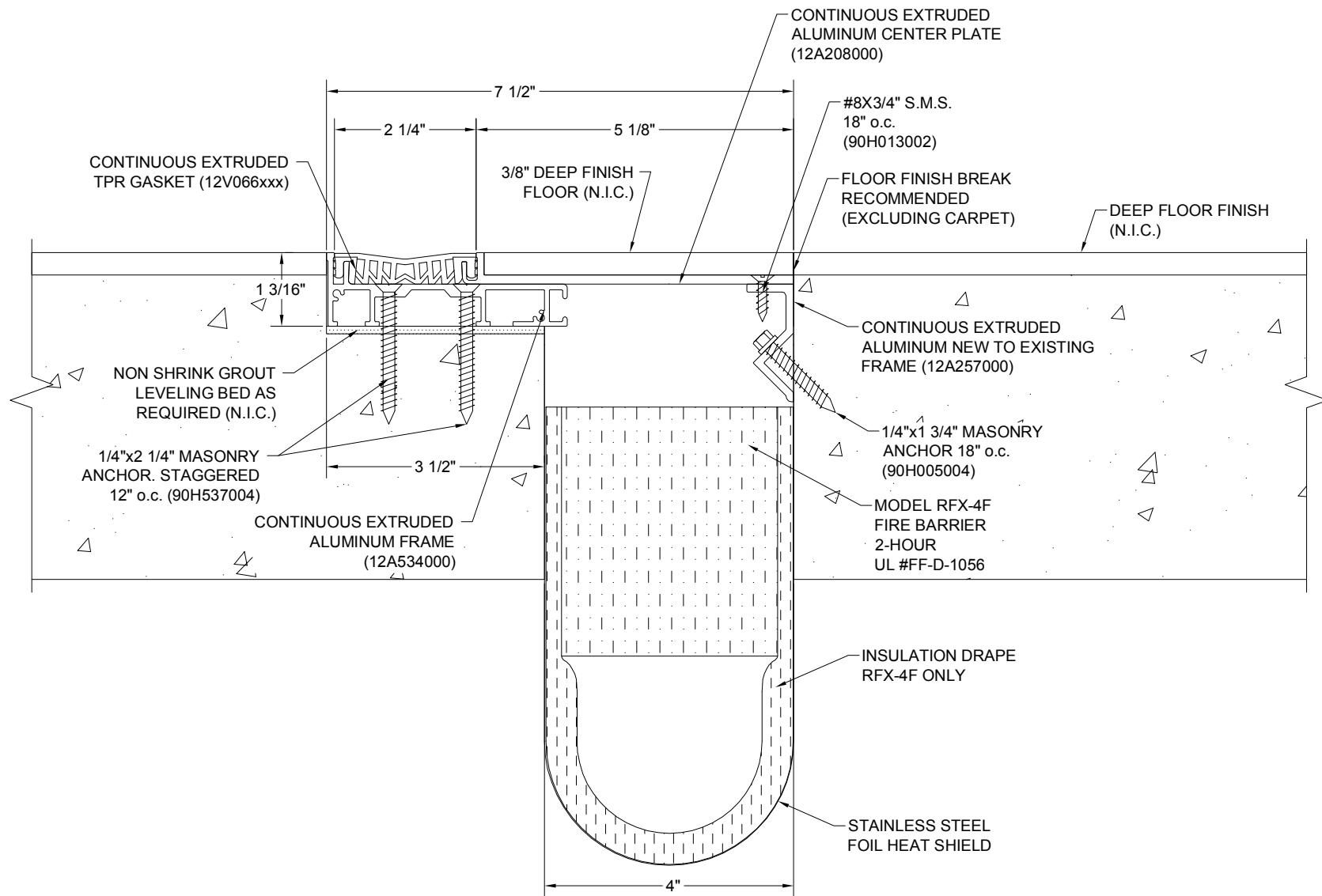
DGTR-400DM w/ RFX4F
