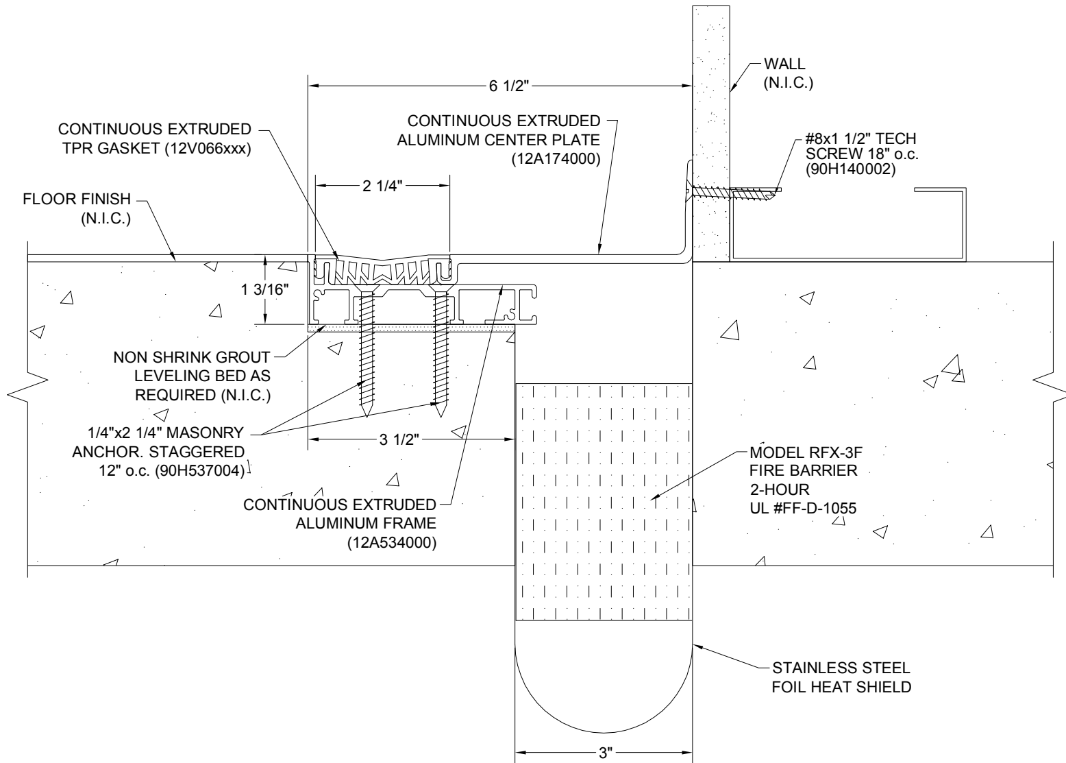
DGTPW-300 w/ RFX3F
