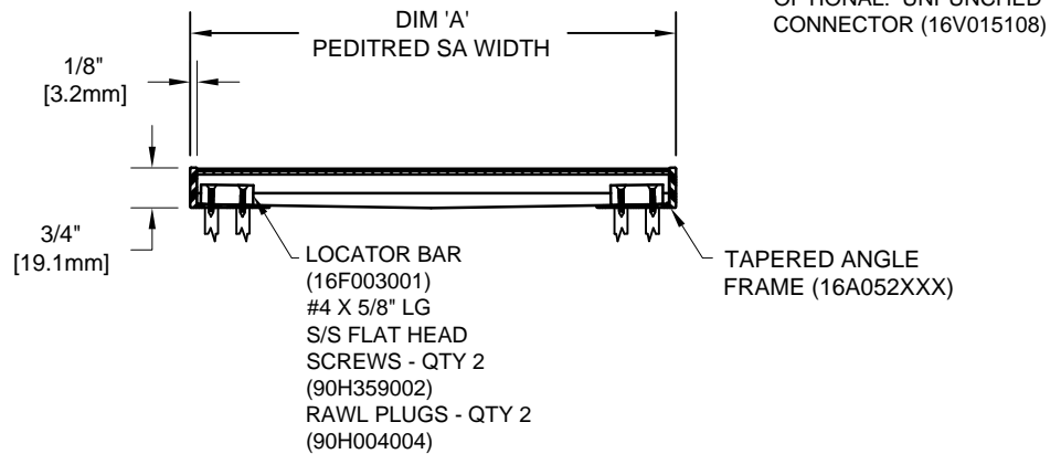
SECTION X-X
