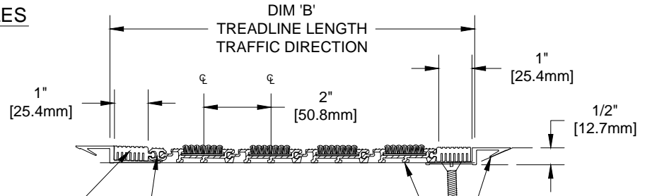
SECTION Y-Y
