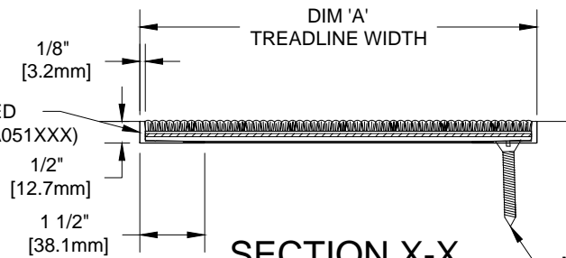
SECTION X-X
