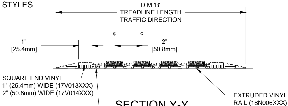
SECTION Y-Y
