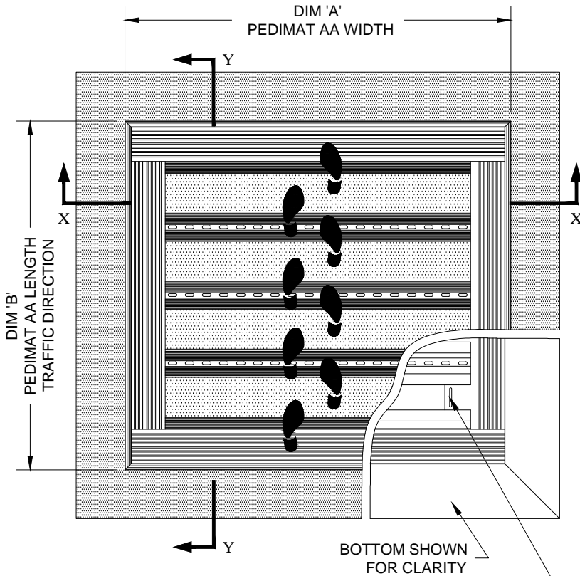
TYPICAL PLAN VIEW
