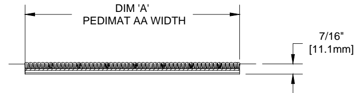
SECTION X-X
