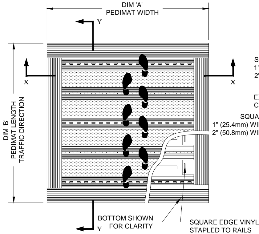
TYPICAL PLAN VIEW
