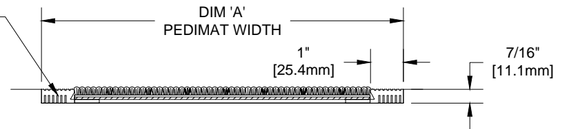
SECTION X-X
