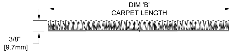
SECTION Y-Y
