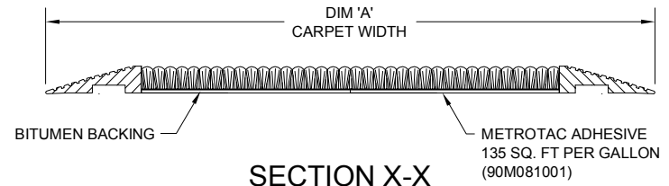
SECTION X-X
