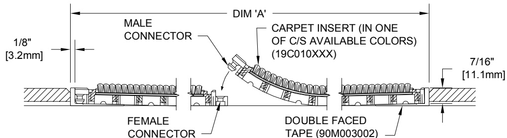
SECTION X-X
