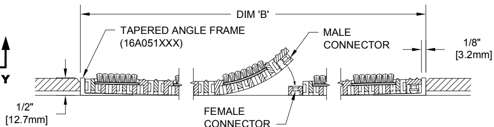
SECTION Y-Y
