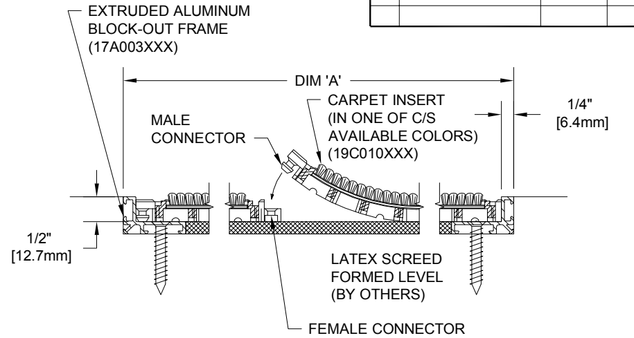
SECTION X-X
