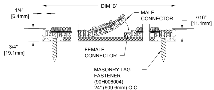
SECTION Y-Y
