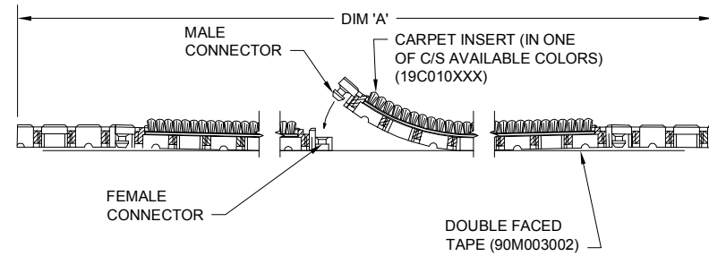
SECTION X-X
