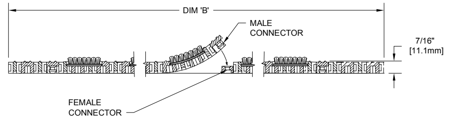
SECTION Y-Y
