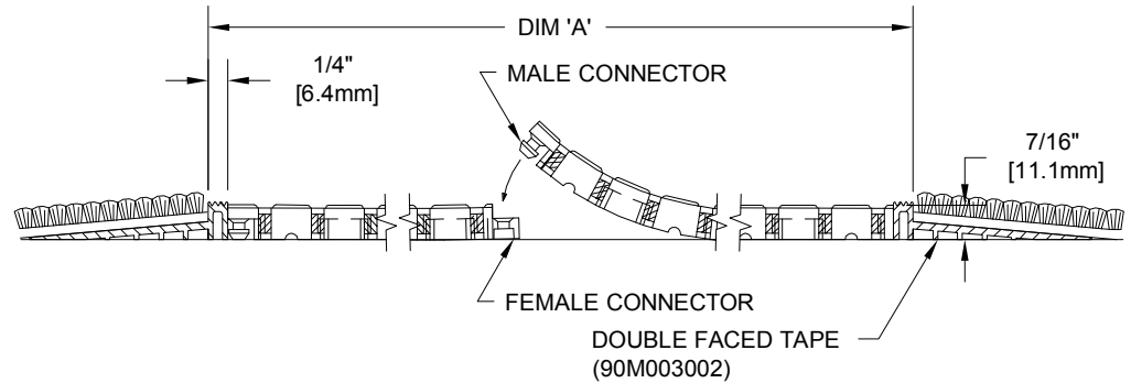
SECTION X-X
