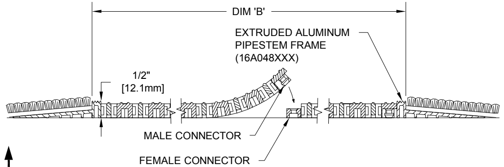
SECTION Y-Y
