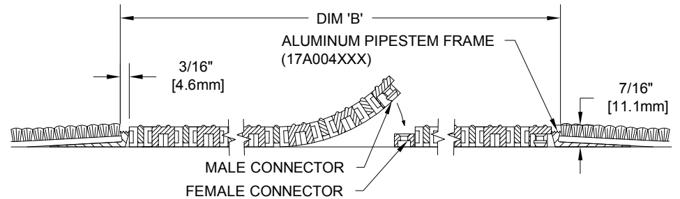
SECTION Y-Y
