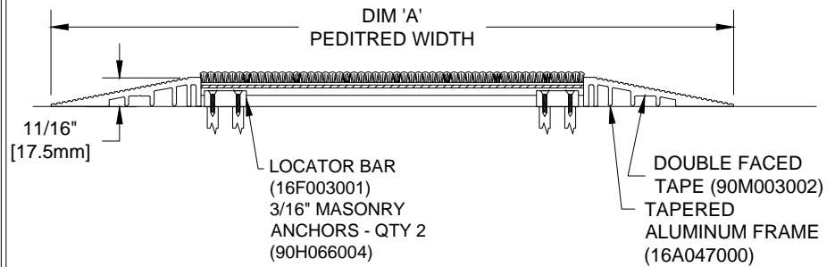
SECTION Y-Y
