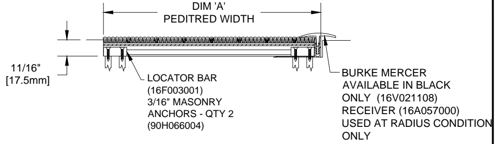
SECTION X-X
