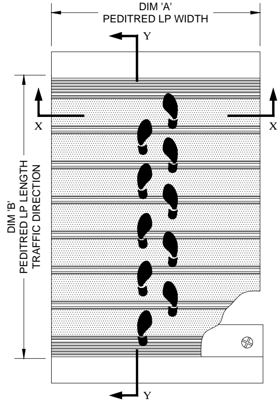
TYPICAL PLAN VIEW
