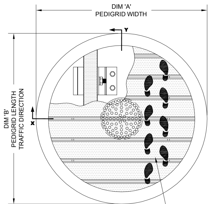
TYPICAL PLAN VIEW PEDIGRID WILL BE SPLIT INTO SECTIONS FOR INSTALLATION
