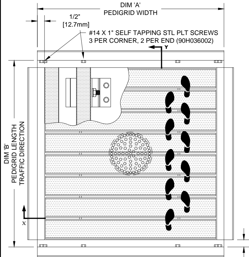
TYPICAL PLAN VIEW
