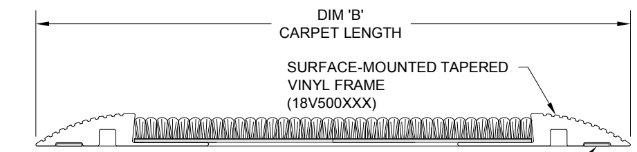
SECTION Y-Y
