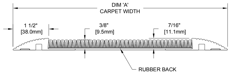
SECTION X-X
