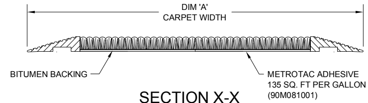
SECTION X-X
