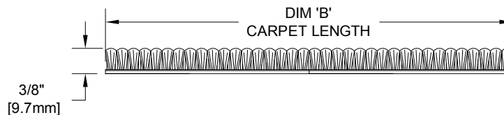
SECTION Y-Y
